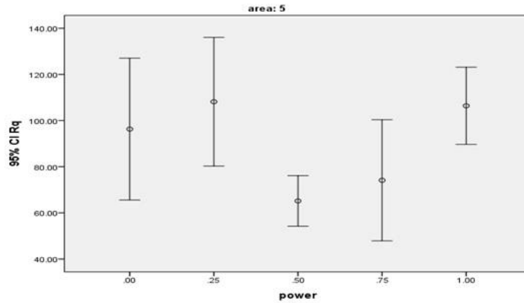
Figure 4. The means and 95% confidence intervals of Rq surface roughness parameter after laser irradiation.
