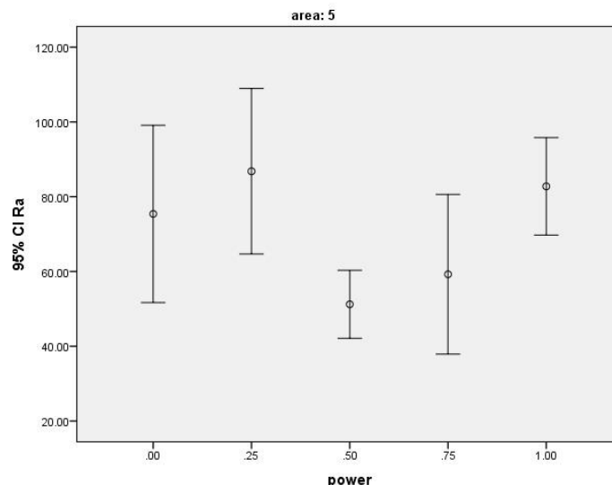
Figure 5. The means and 95% confidence intervals of Ra surface roughness parameter after laser irradiation.
