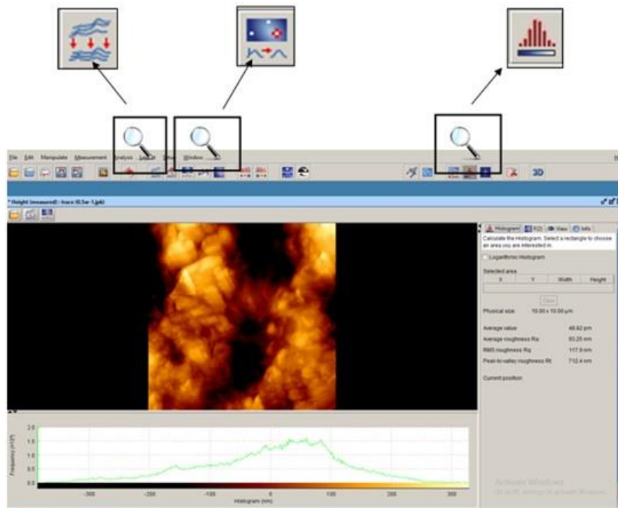
Figure 2. JPK software: Filters used and measurement of surface roughness.
