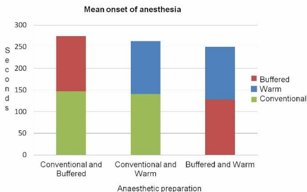
Figure 2: Comparison of mean onset of anaesthesia between buffered, conventional and warm preparations
