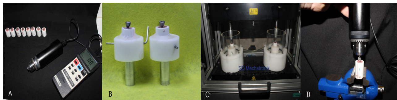
Figure 1. A: Prepared samples and digital torquemeter. B: Samples mounted to be placed in the cyclic loading machine. C: Samples in the cyclic loading machine. D: Measurement of detorque value.
